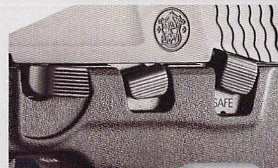
M&P BG380 MANUAL THUMB SAFETY, SLIDE STOP & TAKEDOWN LEVER
