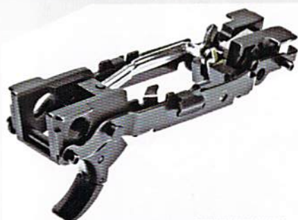
STAINLESS STEEL CHASSIS STEEL-TO-STEEL CONNECTED SYSTEM
